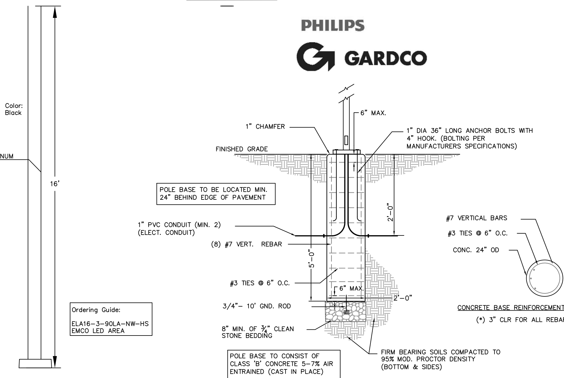
SINGLE LANTERN LIGHT DETAIL NOT TO SCALE
