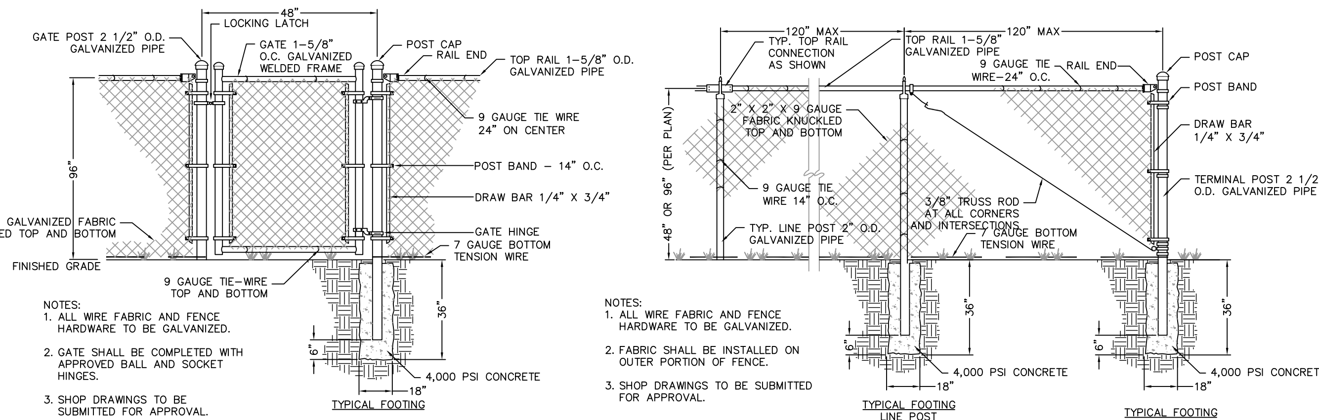
CHAIN LINK FENCE DETAIL NOT TO SCALE
