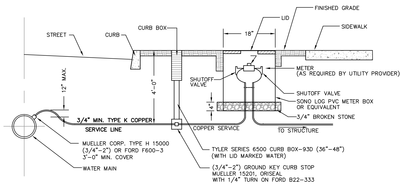
TYPICAL WATER SERVICE DETAIL N.T.S.
