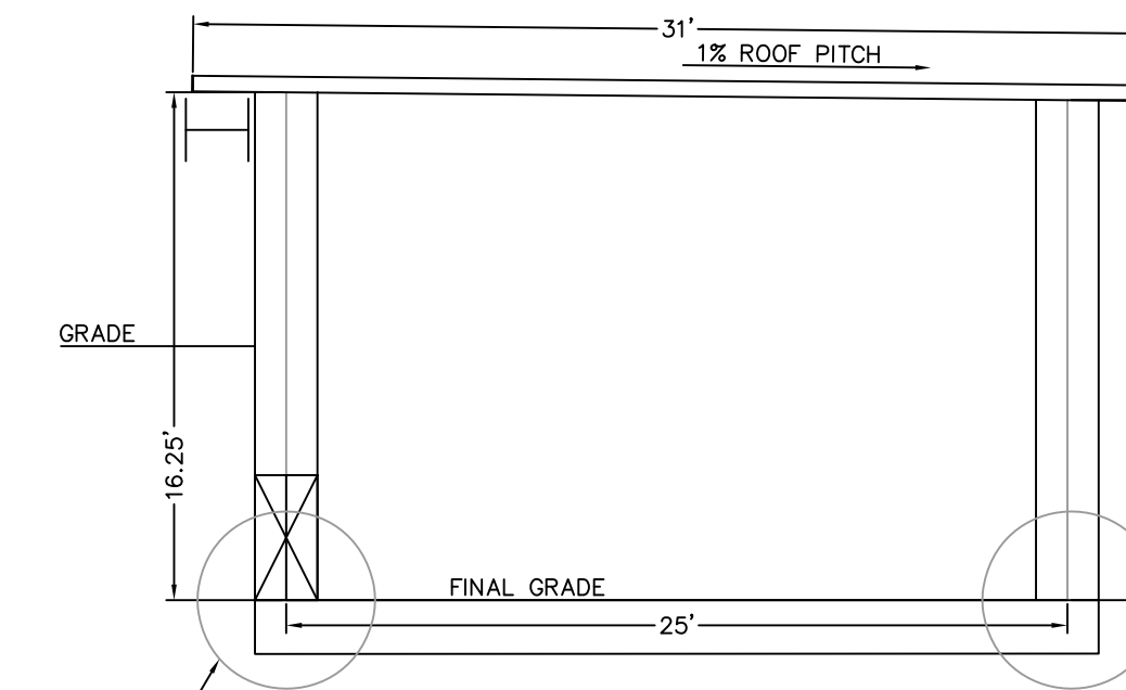
CANOPY STRUCTURAL FRAMING DETAIL NOT TO SCALE
