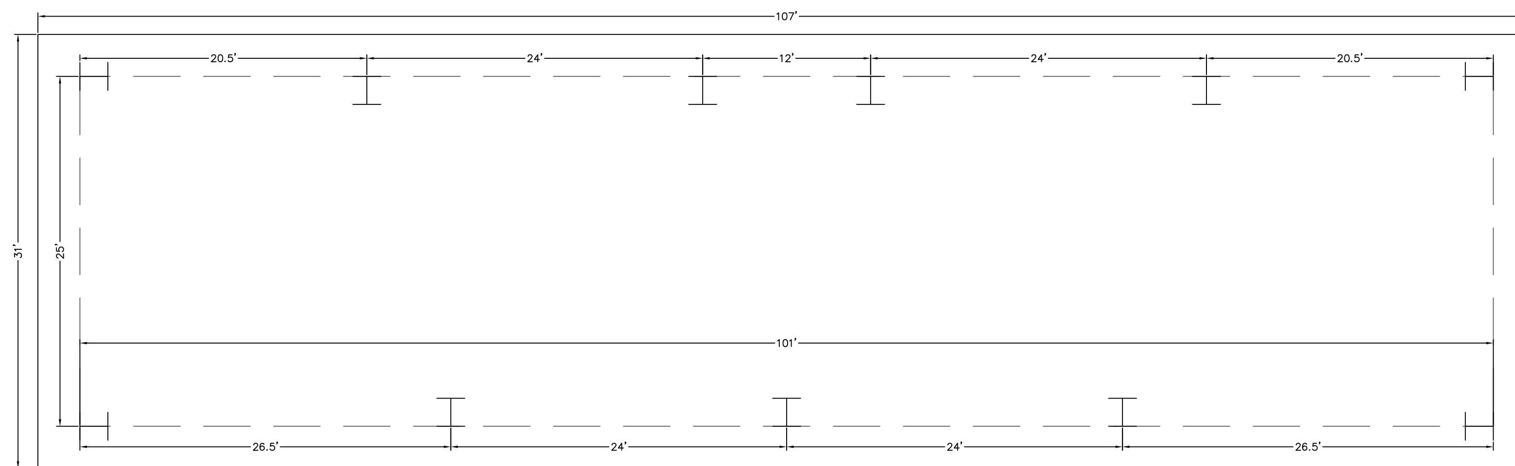
CANOPY PLAN VIEW AND POST SPACING DETAIL NOT TO SCALE
