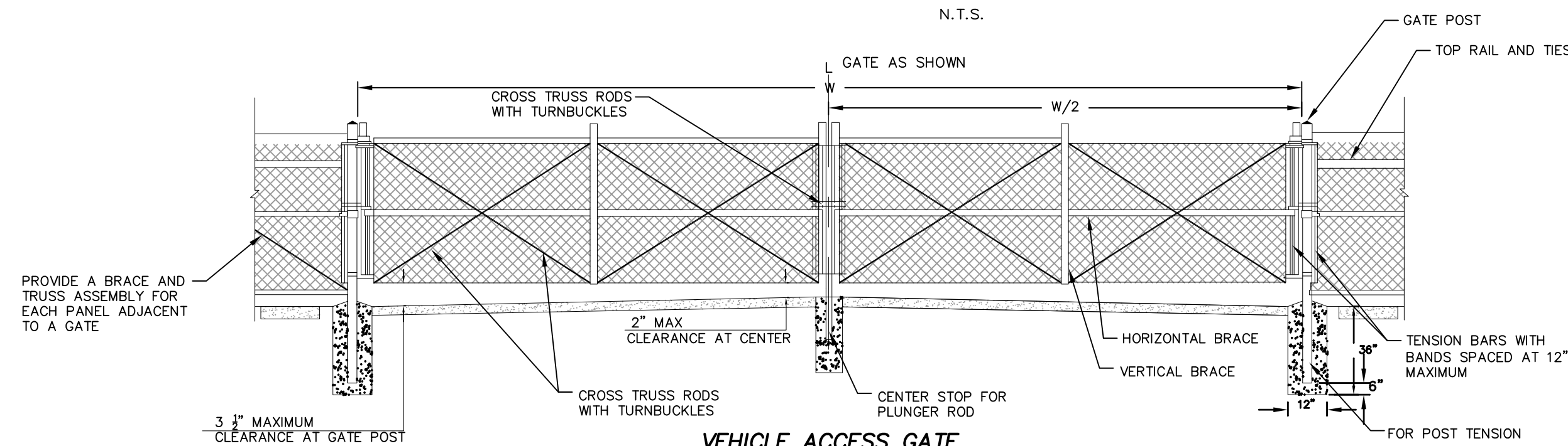
VEHICLE ACCESS GATE NOT TO SCALE
